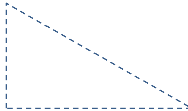
Right Triangle
