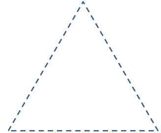
Equilateral Triangle
